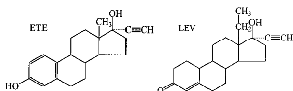
Figure 1- Structure of levonorgestrel and ethinyloestradiol.
