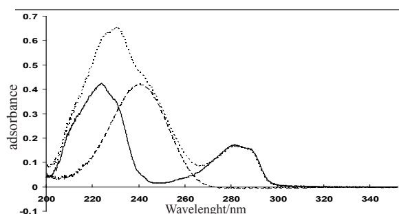
Figure 2- Absorption spectra of ethinylestradiol (—) 25 \mu\text{g ml}^{-1} , levonorgestrel (---) 8 \mu\text{g ml}^{-1} and their mixture (...).
