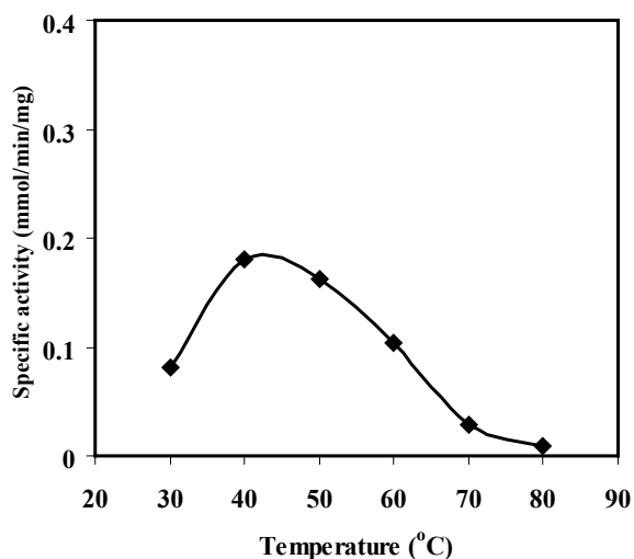
Fig. 2. Effect of temperature on purified xylanase.
