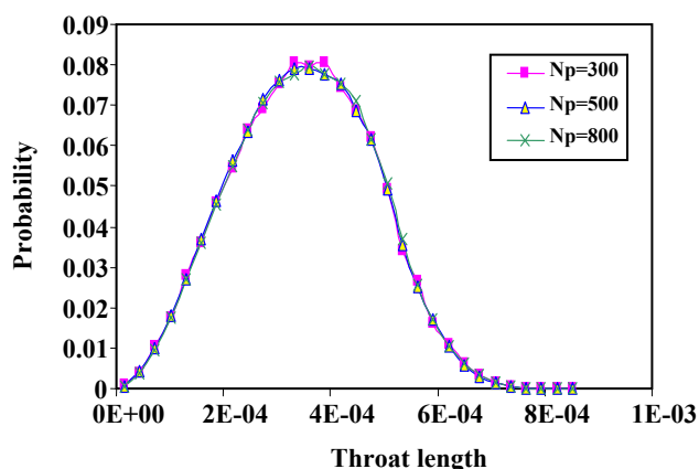
Fig. 3: Effect of N_p in throat length probability distribution in a fixed volume.
