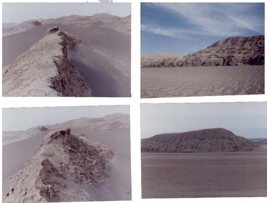
Figure 2. Some important land cover types of the yardang region in the Lut Desert.
