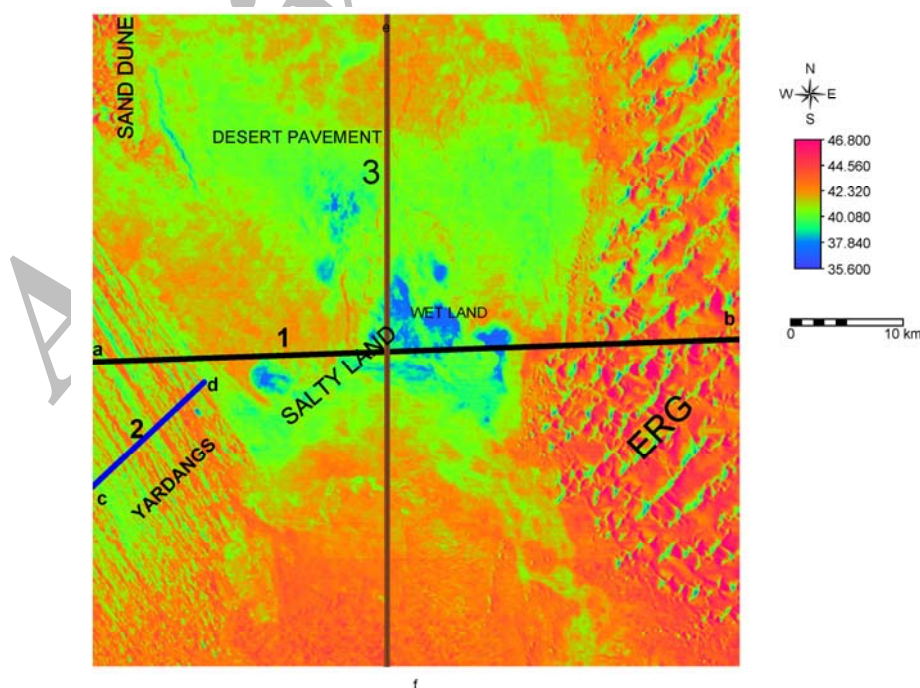
Figure 9. Highlighted surface temperature distribution in the Lut Desert derived from the TM band 6 image data and cross-section.
