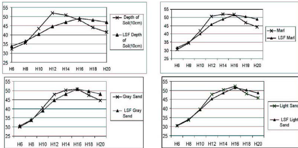
Figure 4. The comparison of real temperature and estimated temperature according to Least Square Fitting (LSF), Y-axis presents temperature in Celsius ( ^{\circ}\text{C} ) and X-axis also presents times in every two hours during a day between 6 a.m. until 8 p.m..
