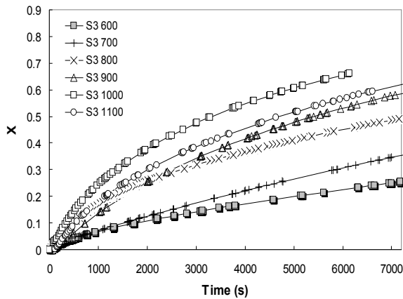
Figure 7. Weight loss versus time for S3.
