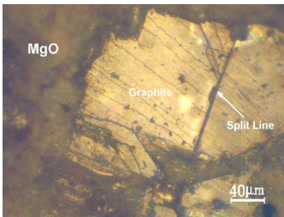
Figure 4. Optical-microscope image of a large graphite flake seen on the cross section of the S0 sample. The initial flake size is around 420×480 µm
