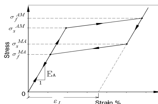
Fig. 1. Stress-strain curve for SMA.
