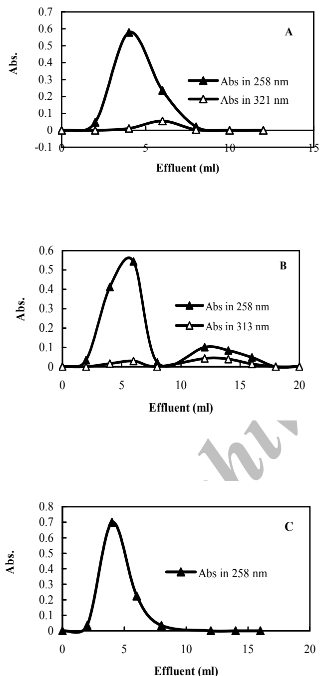
Fig. 10. Gel chromatograms of (A) [\text{Pt}(\text{bpy})(\text{Et-dtc})]\text{NO}_3 -DNA complex, (B) [\text{Pd}(\text{bpy})(\text{Et-dtc})]\text{NO}_3 -DNA complex and (C) only DNA, obtained on Sephadex G-25 column, equilibrated with 10 mM Tris-HCl buffer of pH 7.0 in the presence of 0.01 M sodium chloride.
