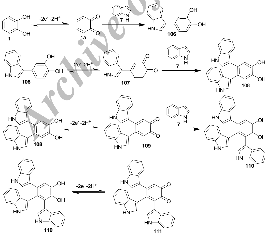
Scheme 32
