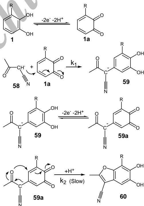
Scheme 20
