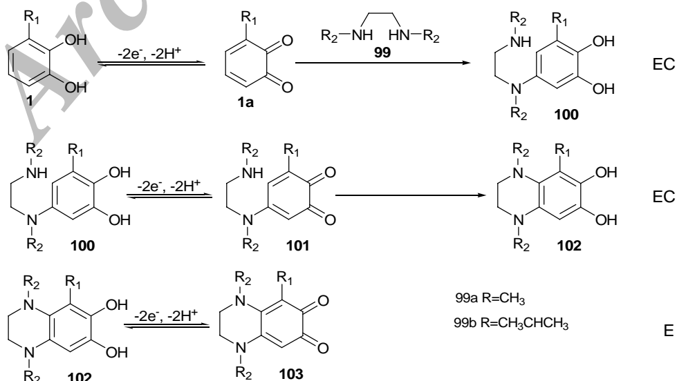
Scheme 30
