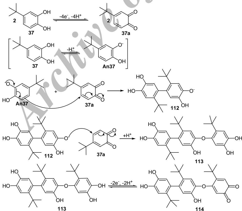
Scheme 33
