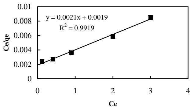
Fig. 12. Langmuir Isotherm for adsorption of MG on mesoporous carbon adsorbent.
