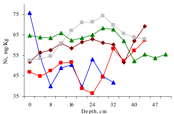
Fig. 5: Distribution of Ni in sediment cores
