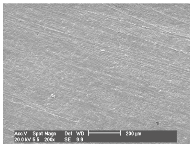
Figure 6. SEM of a silver deposit on the Cu backing grown at a current density of 4.27 \text{ mA.cm}^{-2} from 5.16 \text{ g l}^{-1} Ag CN, 5.16 \text{ g l}^{-1} KCN, 3 \text{ g l}^{-1} \text{Na}_2\text{CO}_3 solutions, \text{pH}=12 , 40^\circ\text{C} , 133mm thickness.
