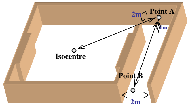
Figure 1. Simulated treatment room geometry and points A and B where the neutron and capture gamma calculations were performed.
