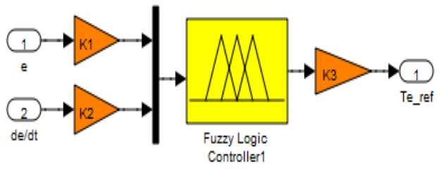
Fig. 8 Bloc diagram of the fuzzy controller.
