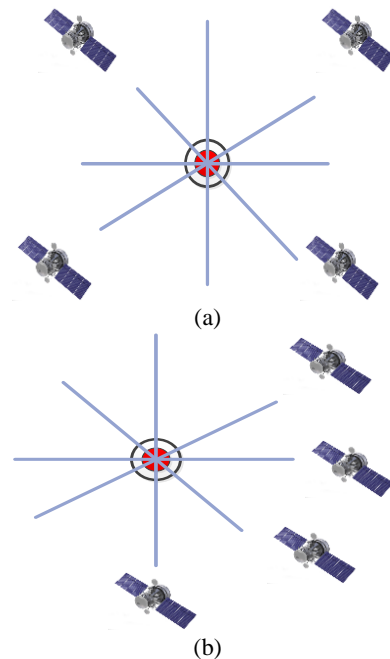
Fig. 1 Satellite geometry representation; a) Good DOP and b) Poor DOP.
