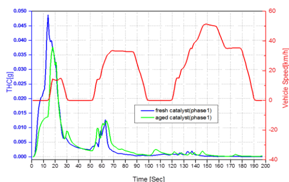
Figure 15: The concentration of THC during first stage of NEDC cycle.
