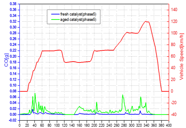
Figure 11: The concentration of CO during last stage of NEDC cycle.
