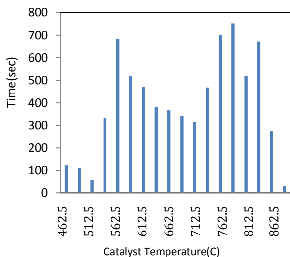
Figure 5: Quality Metric Histograms of vehicle catalyst temperature on SRC cycle.
