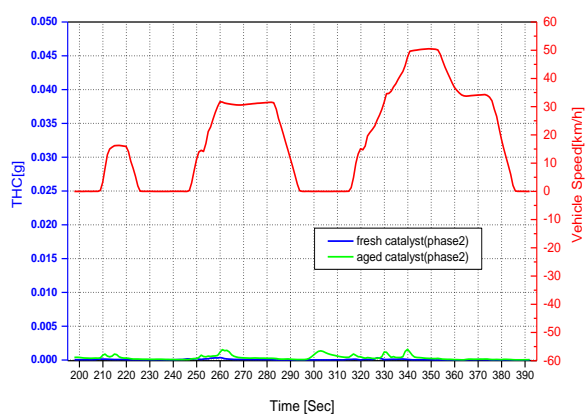
Figure 16: The concentration of THC during second stage of NEDC cycle.
