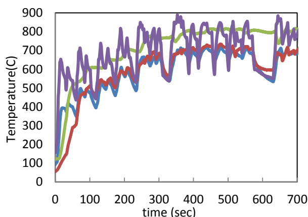
Figure 6: vehicle catalyst temperature on SRC cycle (in different position of catalyst).
