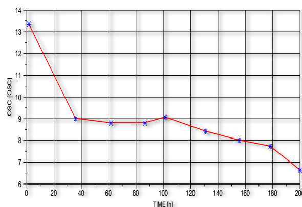
Figure 7: The oxygen storage capacity at different times of the aged catalyst from fresh.
