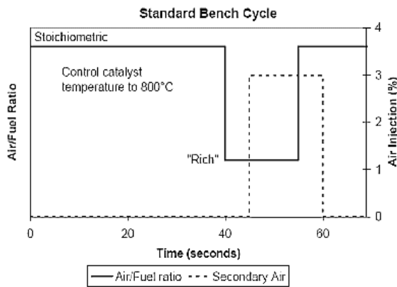
Figure 2: The Standard Bench Cycle used for accelerated aging of the catalyst [9].
