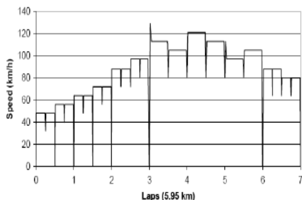
Figure 4: The standard road cycle used for accelerated aging of the catalyst [9].
