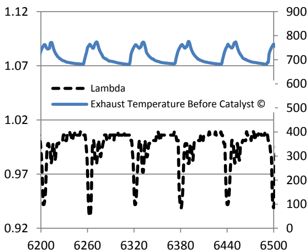
Figure 3: The Standard Bench Cycle used for accelerated aging of the catalyst.
