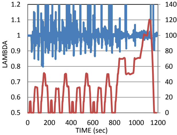
Figure 8: The lambda variation during the NEDC cycle.
