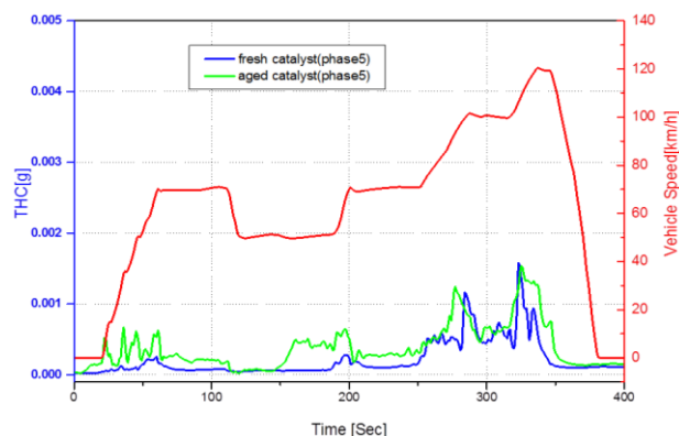
Figure 17: The concentration of THC during last stage of NEDC cycle.
