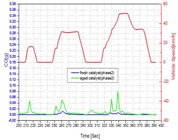
Figure 10: The concentration of CO during second stage of NEDC cycle.
