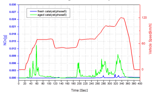
Figure 14: The concentration of \text{NO}_x during last stage of NEDC cycle.
