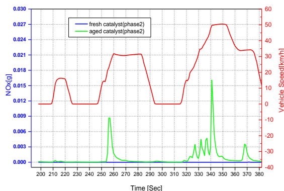
Figure 13: The concentration of \text{NO}_x during second stage of NEDC cycle.
