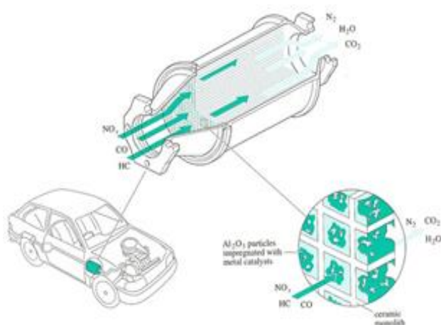
Figure 1: Schematic diagram of the three-way catalytic converter.
