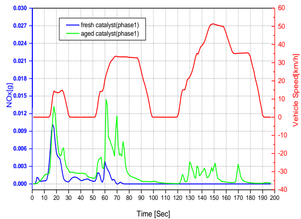
Figure 12: The concentration of NO x during first stage of NEDC cycle.
