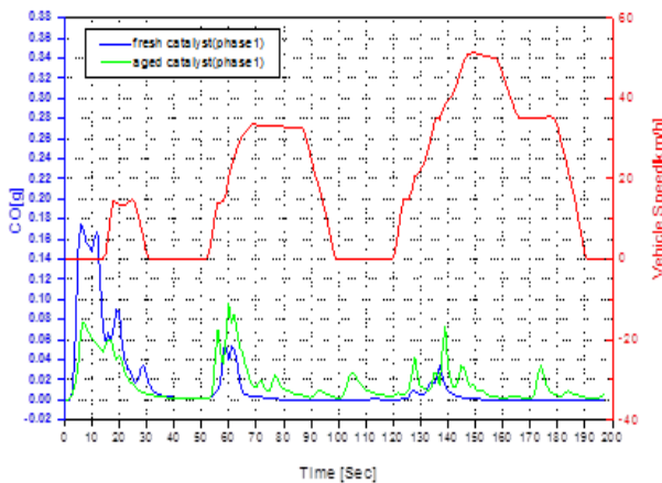
Figure 9: The concentration of CO during the first stage of the NEDC cycle.
