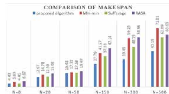
Fig. 2. Makespans for Fixed resources and Varying tasks Makespans of the algorithms.
