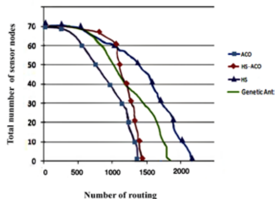
Fig. 3. The life trend of the entire network
