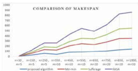
Fig. 3. Makespans for varying resources and Varying task Makespans of the algorithms
