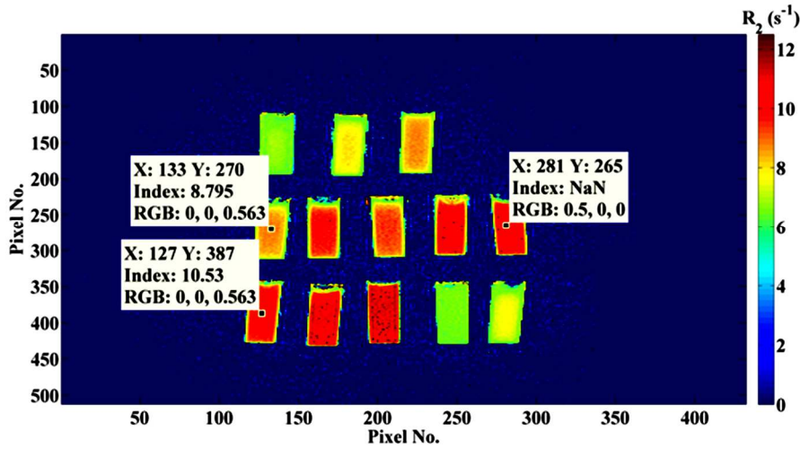
Figure 1. The R_2 map of the PAGATUG polymer gel dosimeter obtained from a sequential signal intensity with ES=22ms. Data cursors on some points are exhibited. The corresponding R_2 values of some pixels are represented as “index” value.
