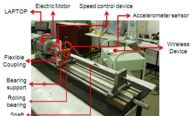
Fig. 8 Shaft experimental setup
