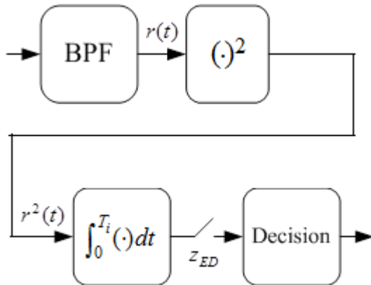
Fig.1. Block diagram of energy detector.
