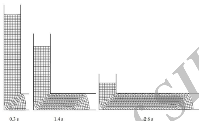
Fig. 2. Element distortion during ECAP
