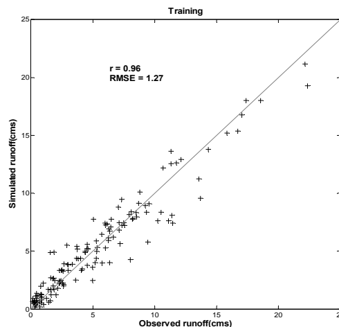
Fig 3. Observed versus simulated runoff for training period.
