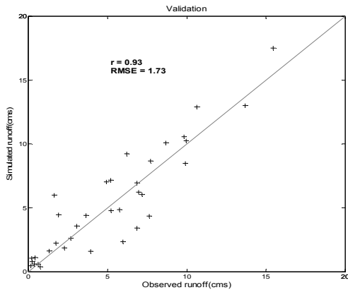
Fig 4. Observed versus simulated runoff for the validation period.
