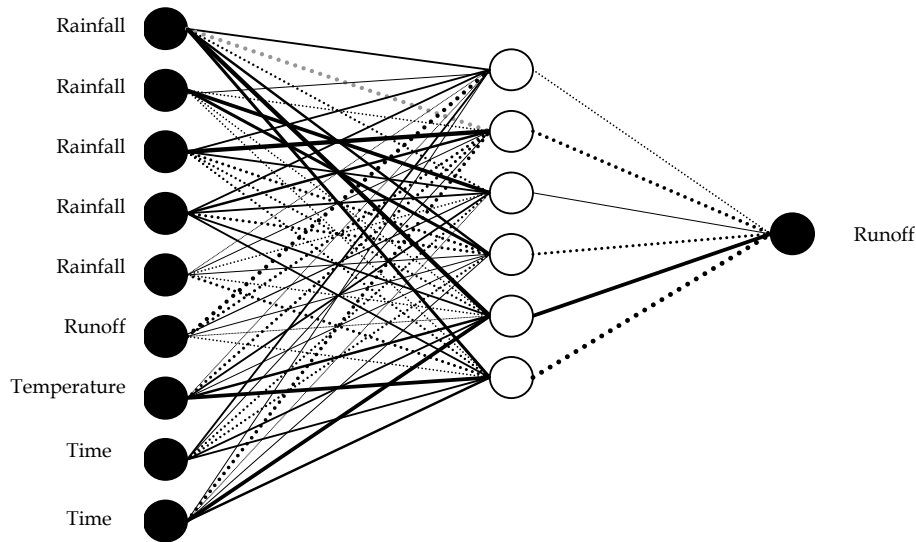
Fig 5. Neural Interpretation Diagram (NID) for artificial neural network (ANN) rainfall-runoff modelling. The line thickness represents the magnitude of the connection weights and the format of the lines as dotted (negative effect), and solid (positive effect) represents the direction of the connection weights.
