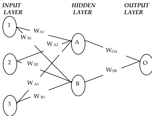
Fig 2. An ANN structure for the illustration of Garson's algorithm.
