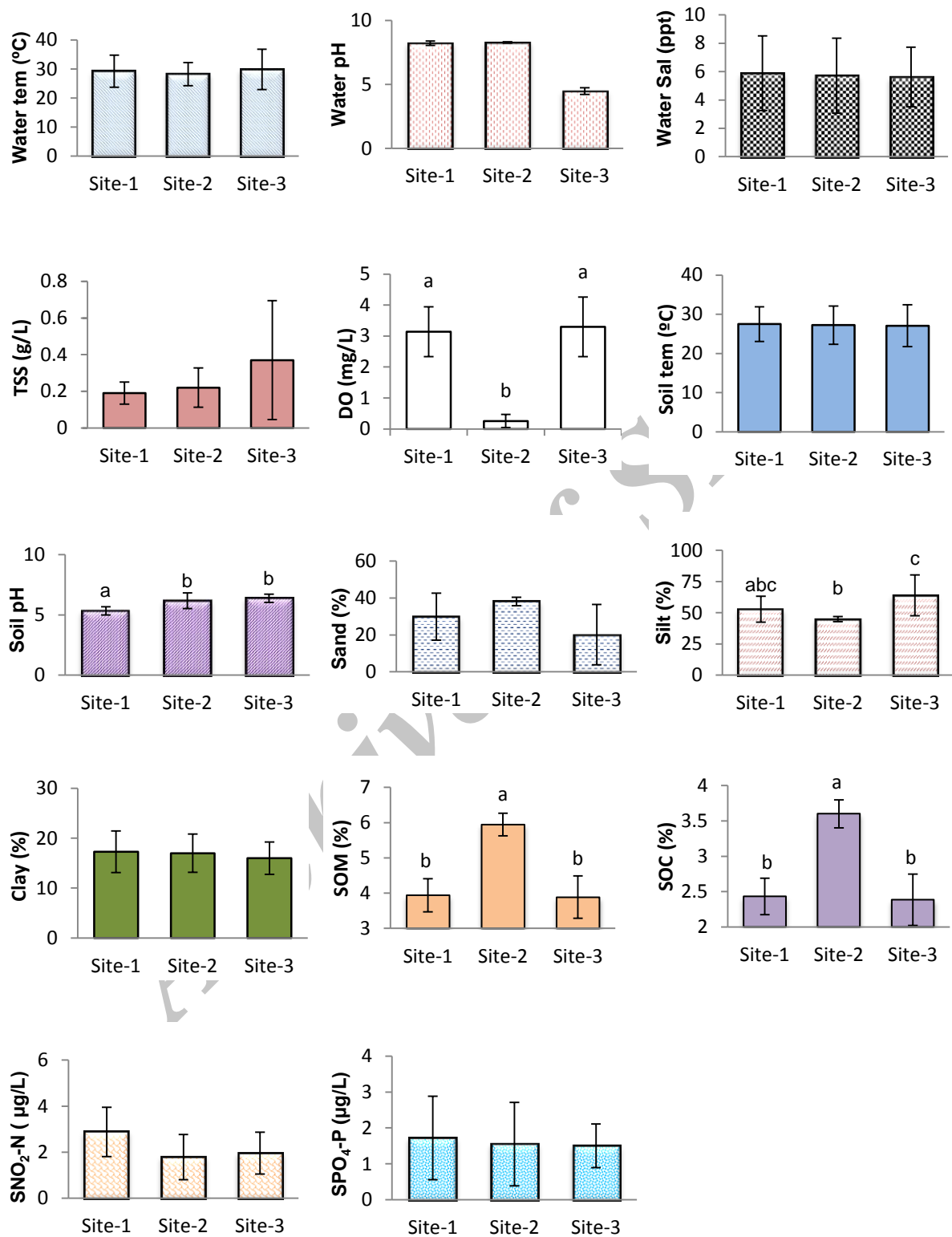
Fig. 2. Spatial variation (Mean±SD) of water and sediment quality parameters. Bars with the same letter are statistically indifferent.
