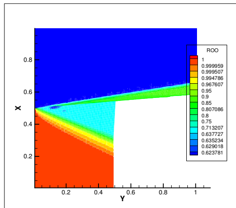
Fig. 6. Density contour
