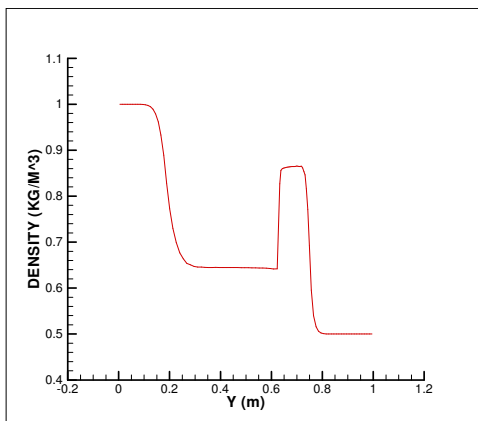
Fig. 3. Density distribution [7]
