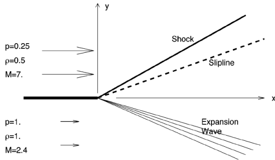
Fig. 1. View of a steady two-dimensional Riemann problem [5]
