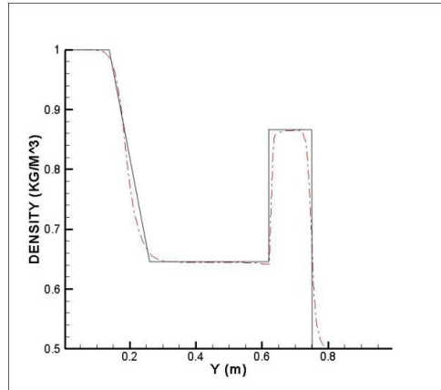
Fig. 4. Comparison of calculation results with the exact solution (continuous line: exact solution, dash lines: Unified coordinates calculation) [7]
