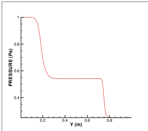
Fig. 2. Pressure distribution [7]
