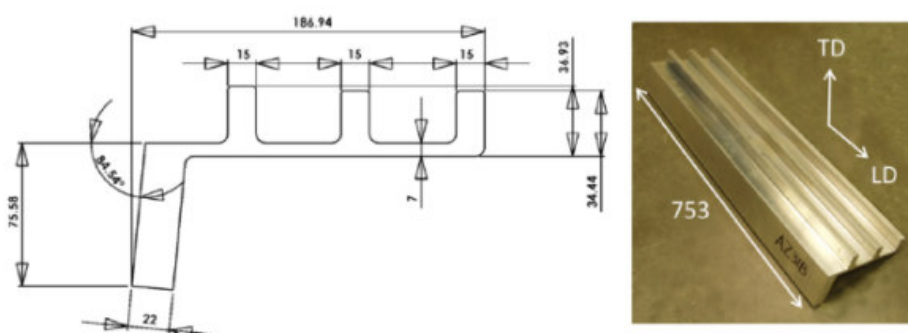
Fig. 3. AZ31B extrusion. All dimensions in mm [4].
