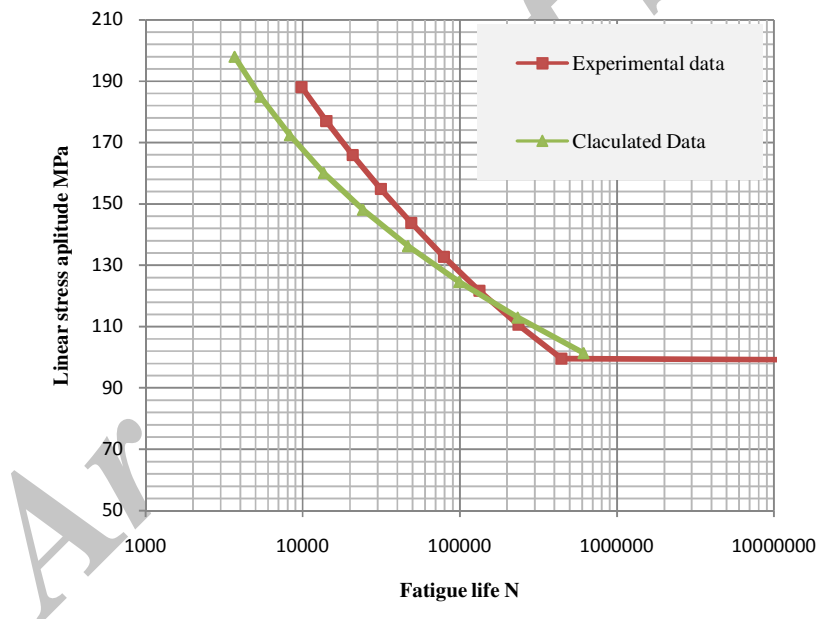
Fig. 9. S-N curve of AZ31B alloy.
