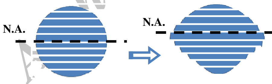
Fig. 2. Changes in elements' shape and the position of the neutral axis.
