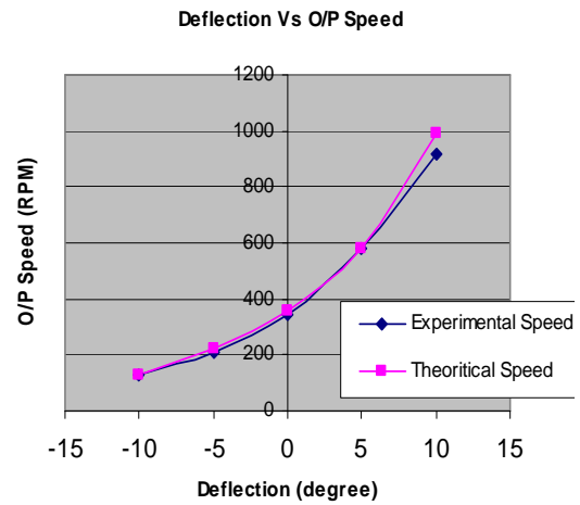
Fig. 9 Deflection Vs O/P speed
