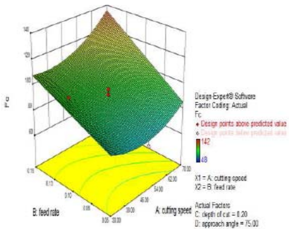
Fig. 10 The 3D response plot for tangential force ( F_c , N) according to change of depth of cutting speed and feed rate with CBN tool
