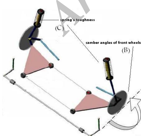
Fig.1 used parameters of front suspension
