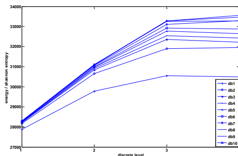
Fig. 5 Total Energy to Total Shannon Entropy ratio for 1~4 decomposition levels of Daubechies mother wavelets
