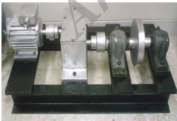
Fig. 1 Fault simulator setup
