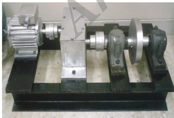
Fig. 1 Fault simulator setup
