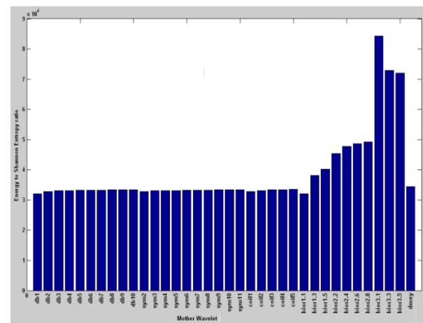
Fig. 4 Total Energy to Total Shannon Entropy ratio for 36 mother wavelet
