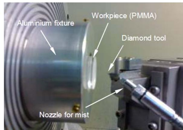
Fig. 2 Close set up view of Diamond Turning Operation
