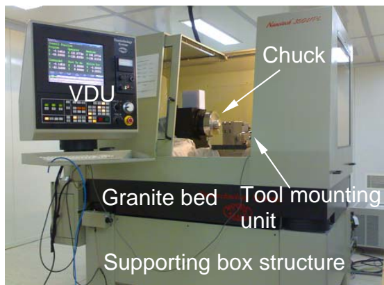
Fig. 1 Diamond Turning Machine
