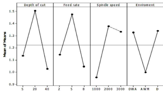
Fig. 5 Main effects plots for flatness in diamond turning of PMMA
