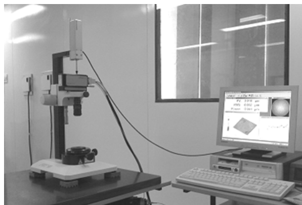
Fig. 3 Optical Interferometer for Diamond Turned Surface Measurement
