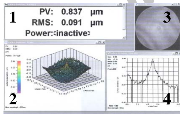
Fig. 4 Flatness Measurement of Diamond Turned Surfaces
