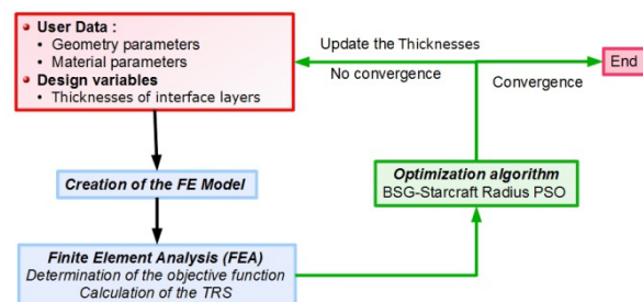
Fig. 3 Optimization process
