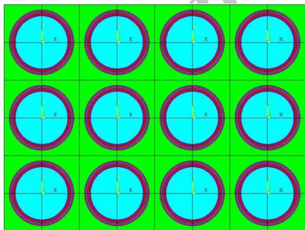
Fig. 1 Transverse cross-section of the 1-D unidirectional C/SiC composites
