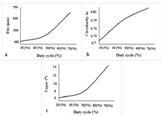
Fig. 7 The influences of duty cycle on hole geometry features
