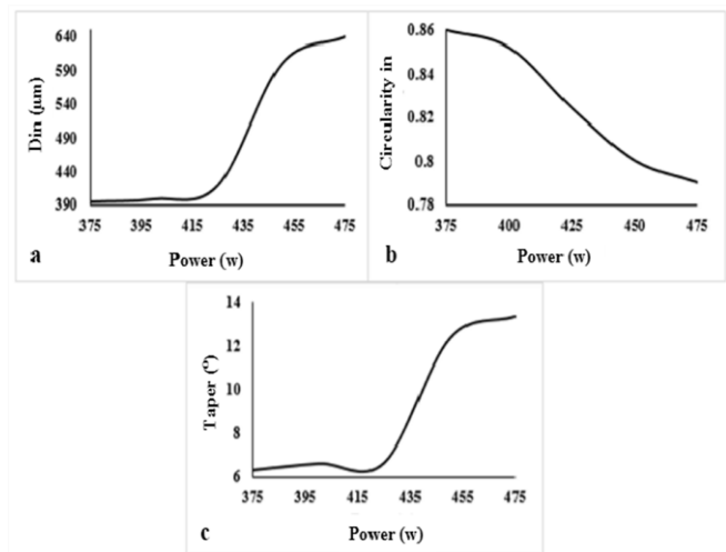
Fig. 6 The Influences of the laser power on hole geometry features
