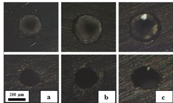
Fig. 4 The Effect of the input parameters variations on profile
