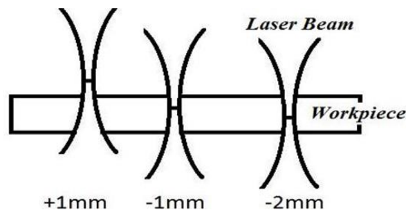
Fig. 3 Variation of focal Plane position on the work piece
