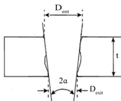
Fig. 1 The geometrical features of cross-section of the hole [15]
