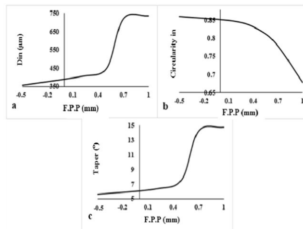
Fig. 8 The influences of focal plane position on hole geometry features
