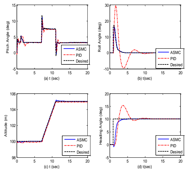
Fig. 9 Nonlinear model variables, PID and ASMC algorithms confrontation
