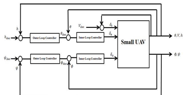
Fig. 2 The control scheme of Small UAV
