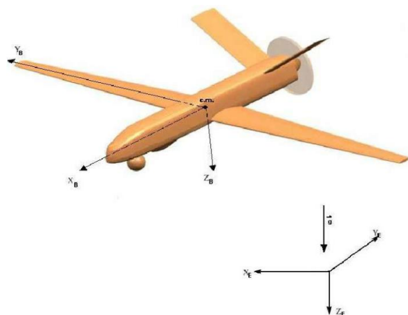
Fig. 1 The Earth-fixed and the Body-fixed coordinate systems [20]
