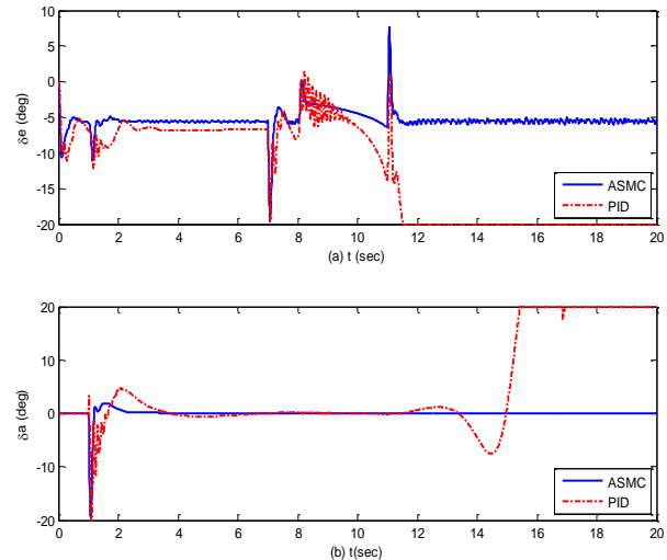
Fig. 14 Nonlinear model control surfaces under uncertainties and disturbance, PID and ASMC algorithms confrontation
