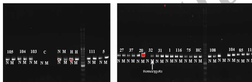
Figure 2. Gel electrophoresis of ARMS PCR for exon 8 of ATP7B gene at T_a of 66°C. Heterozygote samples show normal and mutant PCR bands. Sample with homozygote mutation shows only mutant PCR band (sample 32). N: PCR with normal primer, M: PCR with mutant primer. 50bp DNA ladder is depicted in middle line. H: Heterozygote control, C: Control.
