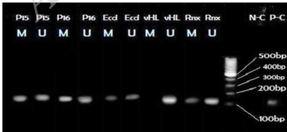
Figure 4. MSP results for studied genes in differentiated cells in presence of EPO
