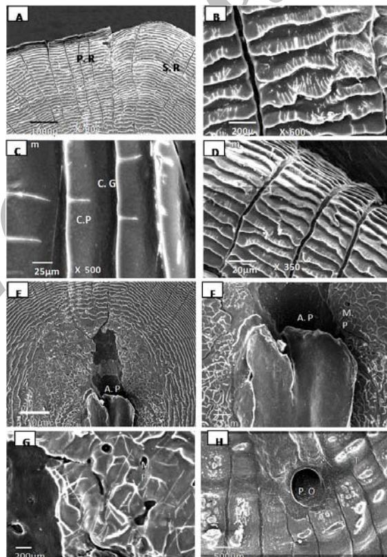
Fig. 5. SEM microphotographs of lateral line scale of C. damascina . radii (R), circuli (C), crest of circuli (C.C), circular groove (C. lateral circuli (l. C), primery radii (P. R), secondary radii (S. R), line of growth (L. G). Anterior pore (A. P), Posterior pore (P. O), Tubercle (T) and Mucus pore (M. P)
