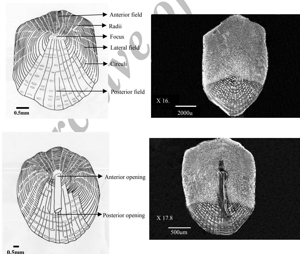
Fig. 3. a) Schematic drawing of a sectioned cyprinid scale. b), SEM microphotograph of a normal C. damascina scale. c) schematic drawing of a sectioned cyprinid lateral line scale. d) SEM microphotograph of C. damascina lateral line scale. Focus (F), posterior opening (PO), anterior opening (AO), posterior field (P), anterior field (A), lateral field (L)
