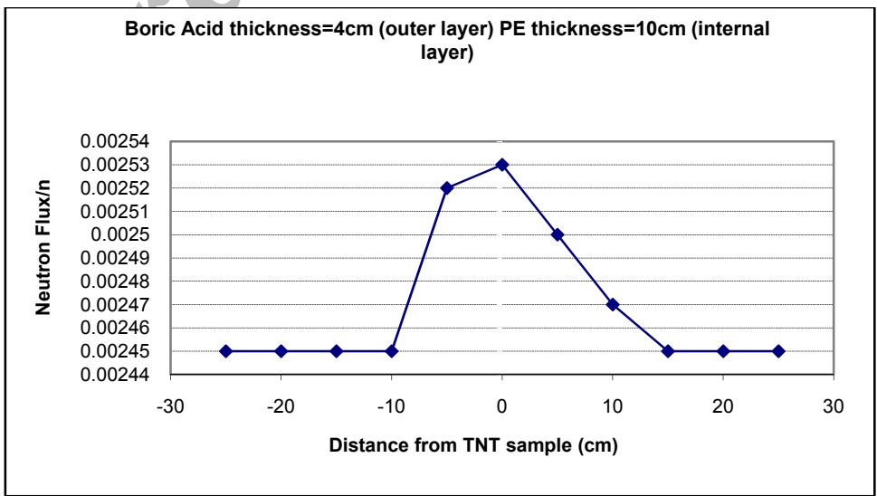
Fig. 5. Backscattered neutron flux with distance from center of TNT sample buried
