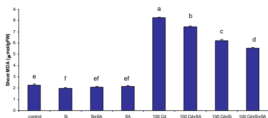
Fig. 5. Effects of Si, Si+SA and SA in the presence and absence of Cd (100 µm) on maize seedlings MDA content
