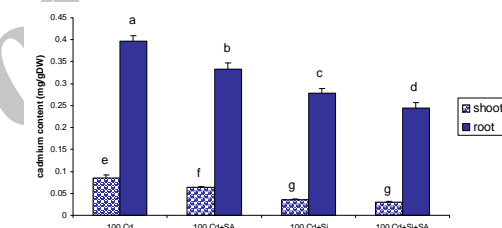
Fig. 3. Effects of SA, Si and Si+SA and on the cadmium content of roots and shoots of maize seedlings (seedling were treated with 100 \mu M Cd)
