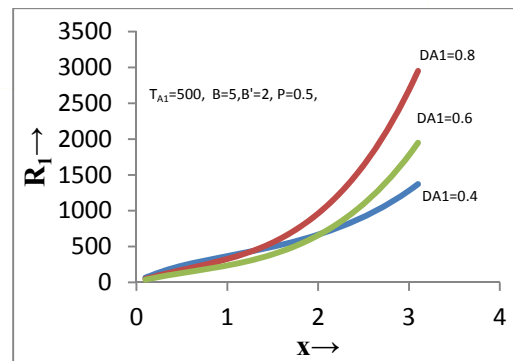
Fig. 4. Variation of Rayleigh number R_1 with dimensionless wave number x for different values of Darcy number D_{A_1}
