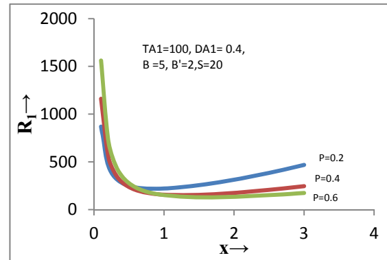
Fig. 6. Variation of Rayleigh number R_1 with dimensionless wave number x for different values of medium permeability P
