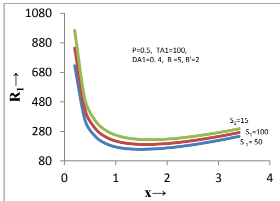
Fig. 2. Variation of Rayleigh number R_1 with dimensionless wave number x for different values of Stable solute gradient S_1
