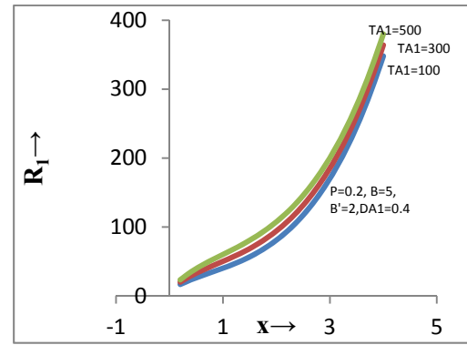
Fig. 3. Variation of Rayleigh number R_1 with dimensionless wave number x for different values of Taylor number T_{A_1}
