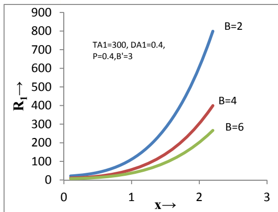
Fig. 5. Variation of Rayleigh number R_1 with dimensionless wave number x for different values of suspended particles parameter B
