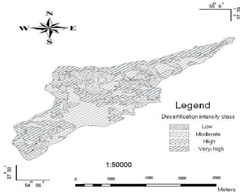
Fig. 4. Map of current desertification status in the study area
