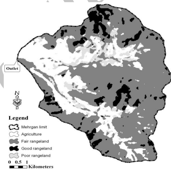
Fig. 7. Land use/cover classification map of study area, using Landsat ETM + 2000
