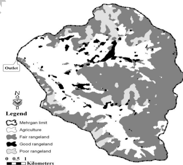
Fig. 8. Land use/cover classification map of study area, using Landsat ETM + 2006
