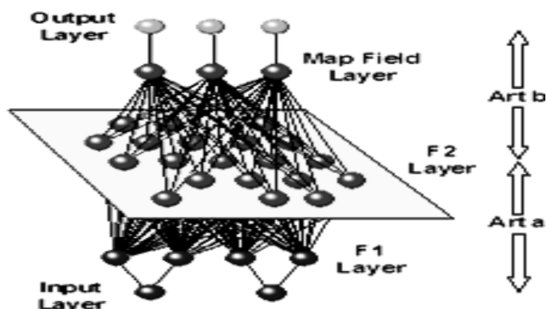
Fig. 5. Training trend in artificial fuzzy ARTMAP neural network (Ronald Eastman, 2009)
