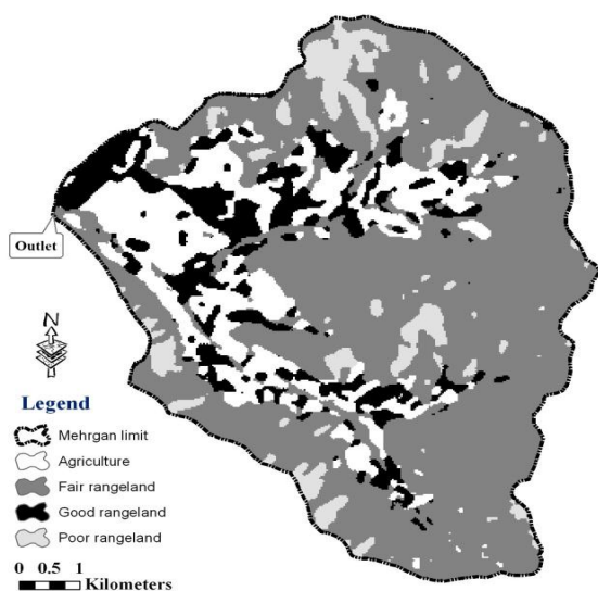
Fig. 6. Land use/cover classification map of study area, using Landsat TM 1987
