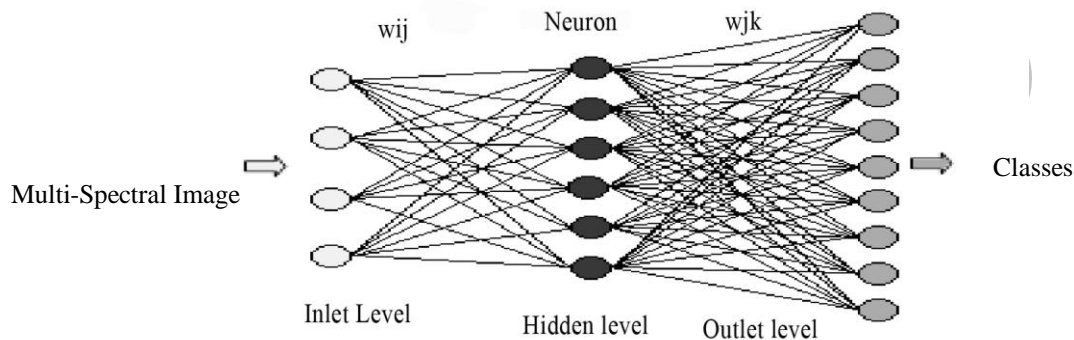
Fig. 4. A simple scheme of neural net model (Carvajal et al. , 2006)
