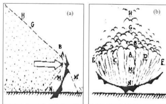
Fig. 1. Sketch from a video capture of (a) the side view (b) and front-view of dust storm peak as a cold front passed through the Hexi Corridor, Gansu March, 2002
