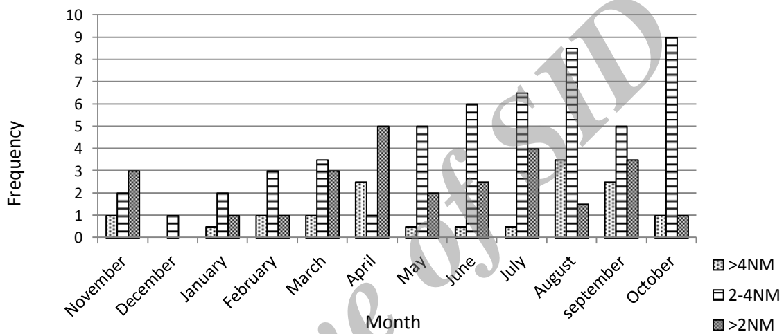
Fig. 3. Monthly Frequency of Dust Storms in Iraq and Kuwait, by Visibility
