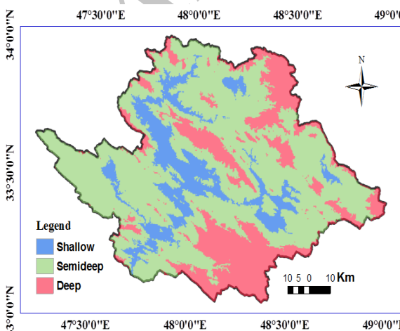
Fig. 4. Groundwater classification
