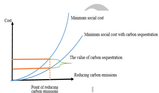
Fig. 3. Social value of carbon sequestration
