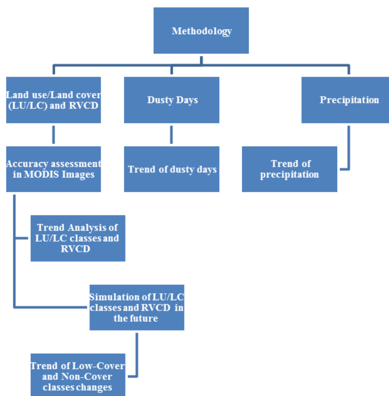
Fig. 2. Schematic Methodology in this research
