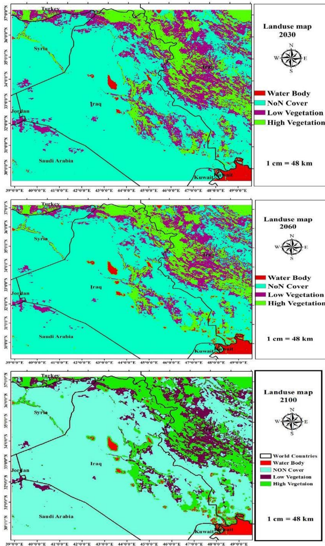
Fig. 4. The predicted LU/LC map of area for 2030, 2060 and 2100
