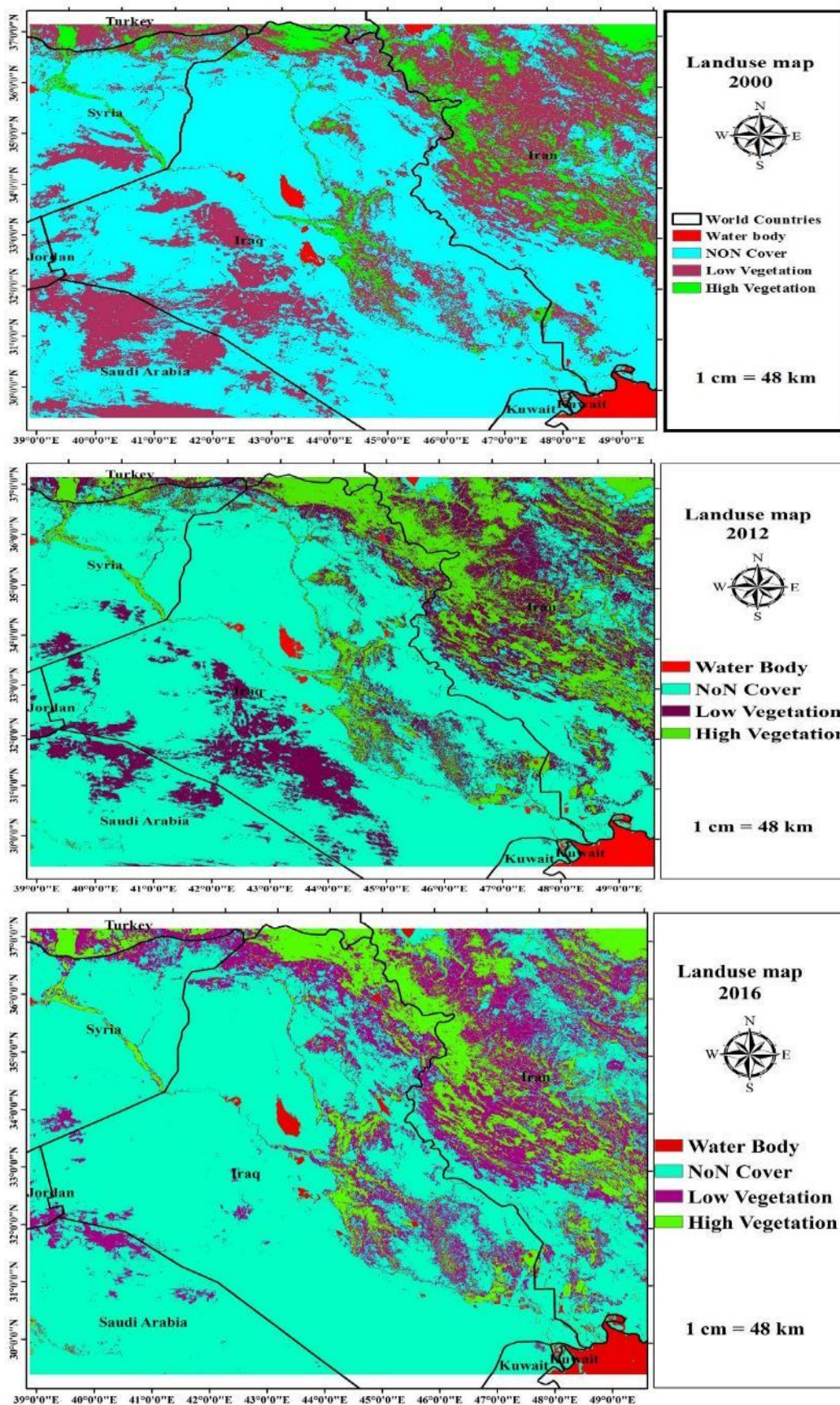
Fig. 3. The observed LU/LC map of area for 2000, 2012 and 2016
