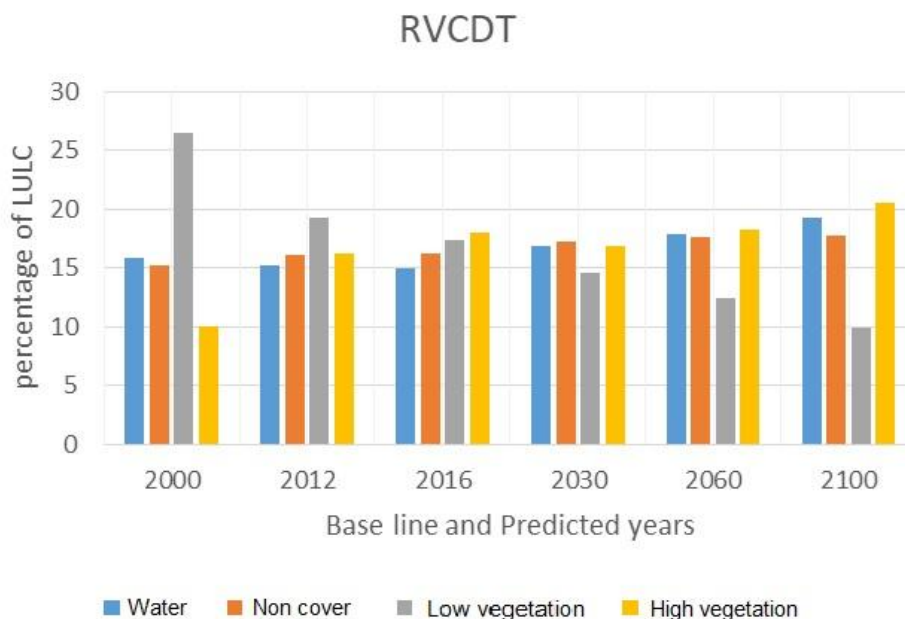
Fig. 5. Regional vegetation cover degradation (RVCDT) and percentage of Land use-land cover (LU/LC) from 2000 to 2100 in the study region
