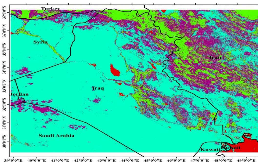
Fig.1. Location of study area in MODIS image
