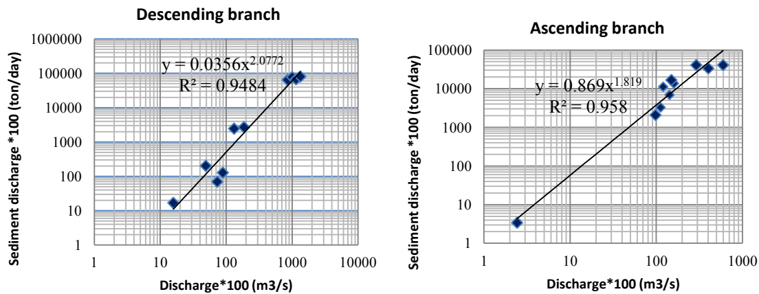
Fig. 5. sediment rating of ascending and descending branches with fitting data average in Manshad watershed (1997-2012).
