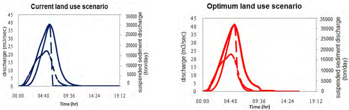
Fig. 8. Comparing estimated hydrograph and sediment graph for return period of 100 years and land use scenarios in Manshad watershed output.
