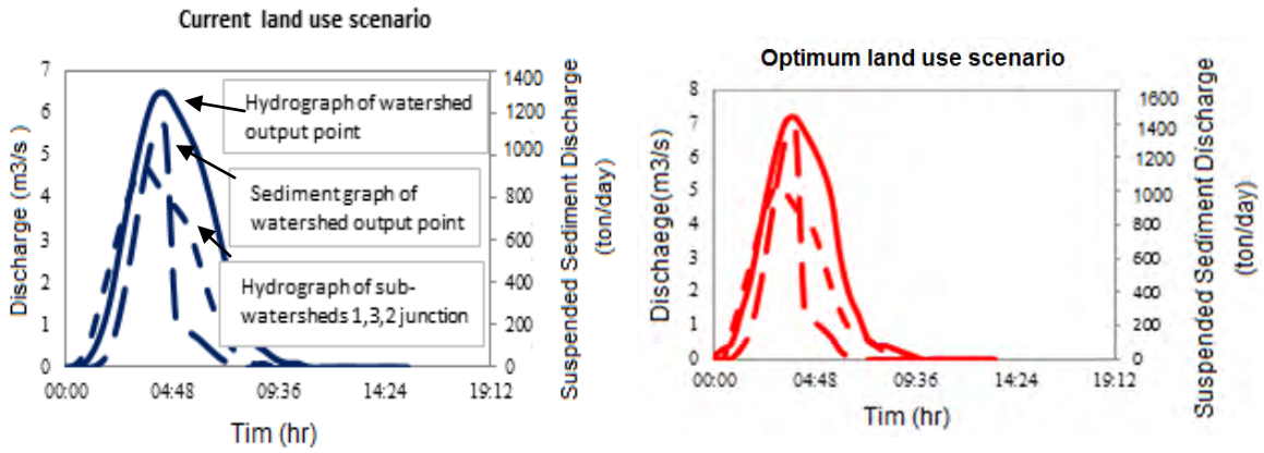
Fig. 6. Comparing estimated hydrograph and sediment graph for return period of 2 years and land use scenarios in Manshad watershed output.
