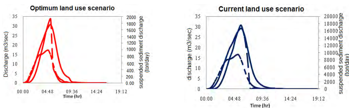
Fig. 7. Comparing estimated hydrograph and sediment graph for return period of 50 years and land use scenarios in Manshad watershed output.
