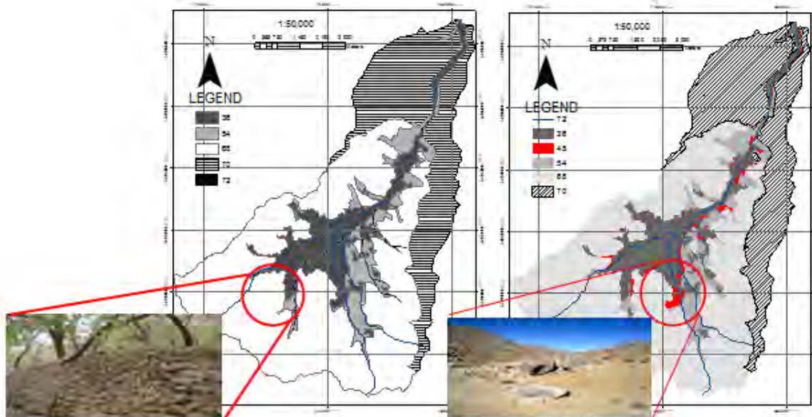
Fig. 4. Curve number of current land use (left) and Optimum land use (right) in Manshad watershed.
