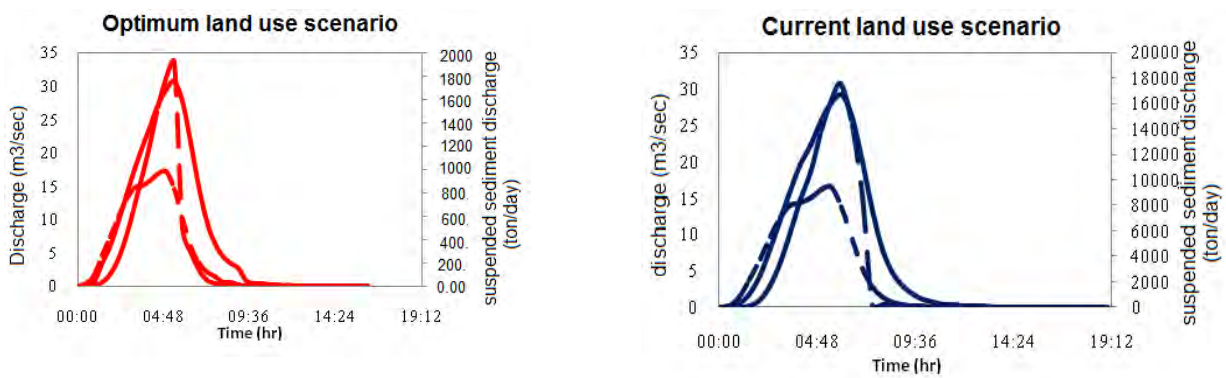
Fig. 7. Comparing estimated hydrograph and sediment graph for return period of 50 years and land use scenarios in Manshad watershed output.
