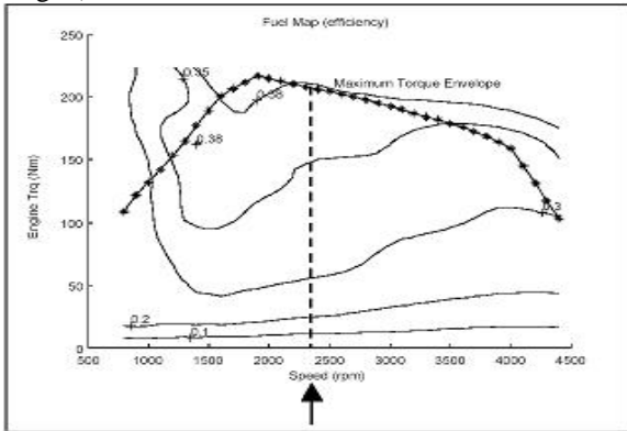
Fig. 6: Engine energy efficiency map
