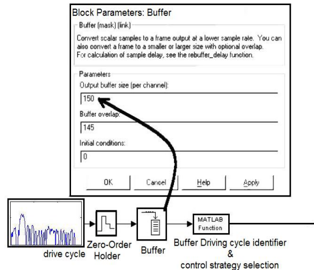
Fig. 12: Control strategy configuration
