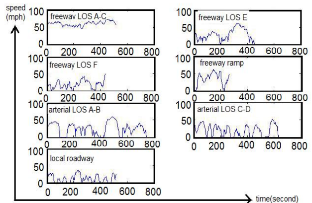
Fig. 1: Facility-specific driving cycles
