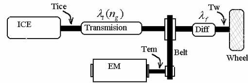
Fig. 5: Mechanical arrangement
