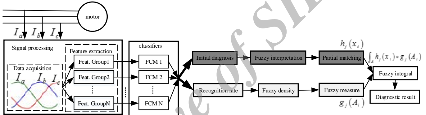
Fig. 4. Structure of decision level data fusion model
