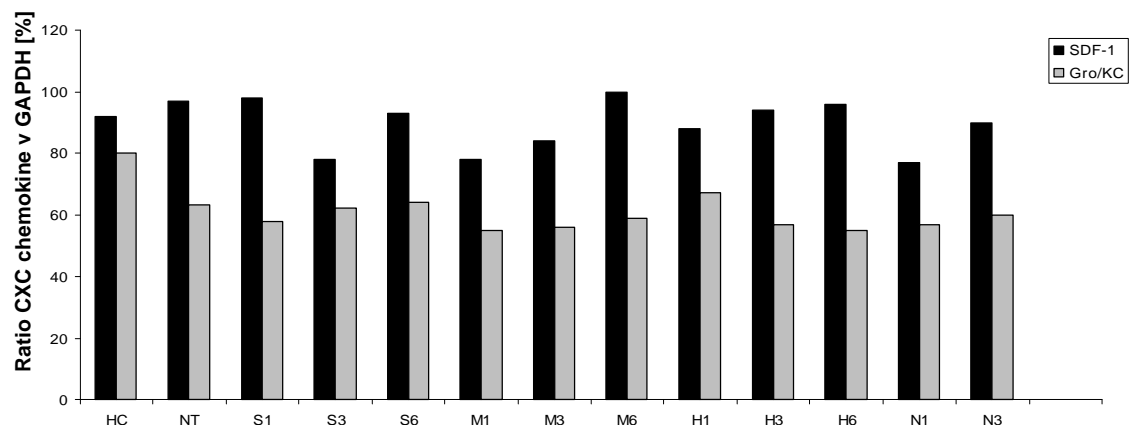
Figure 3. Alteration in expression of CXC chemokines SDF-1 \alpha and Gro/KC against GAPDH in rat's hepatoma H4 cells in different conditions and in the presence and absence of different stimuli. HC=hepatocytes control; NT=not treated; S1=heat shock treatment for 1h; S3=heat shock treatment for 3h; S6=heat shock treatment for 6h; M1=Manitol treatment for 1h; M3=Manitol treatment for 3h; M6=Manitol treatment for 6h; H1=H 2 O 2 treatment for 1h; H3=H 2 O 2 treatment for 3h; H6=H 2 O 2 treatment for 6h; N1=NaCl treatment for 1h; N3= NaCl treatment for 3h.
