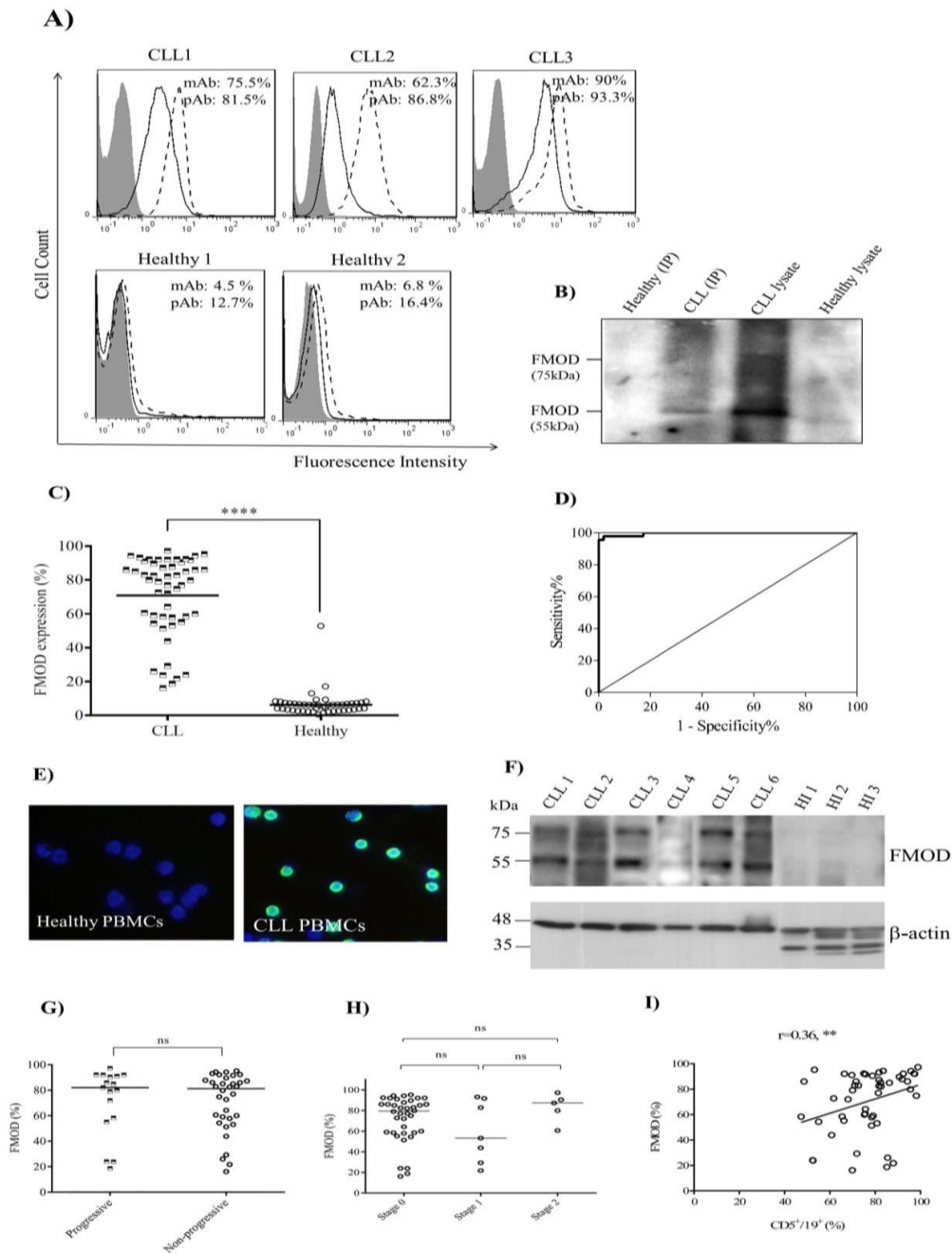
Figure 3. The expression of FMOD in patients with CLL and healthy individuals. A) Detection of FMOD using 2C2 mAb (Solid line) and commercial anti-FMOD pAb (dashed line) in 3 CLL cases and 2 healthy individuals (HI). Gray tinted curve shows detection with isotype control antibodies. B) Immunoprecipitation (IP) was performed to confirm the specificity of 2C2 mAb in detecting FMOD. C) The expression level of FMOD in 52 CLL patients and 45 healthy individuals (****, P<0.0001). D) ROC curve shows the trade-off between sensitivity and specificity for cut-off value of FMOD expression in CLL and healthy samples. E) Immunofluorescent staining showed that 2C2 mAb detected FMOD (green color) in CLL PBMCs, but not in healthy PBMCs. F) Western blot showed that 2C2 mAb detected FMOD in CLL cell lysates but almost not in healthy PBMC lysates. G) No statistically difference in FMOD expression level was identified in CLL patients with progressive or non-progressive form (p>0.05). H) The median expression level of FMOD was not statistically changed in CLL patients with different stages (p>0.05). I) The scatter plot demonstrates a significant correlation (**, P<0.01) between FMOD and CD5 + /CD19 + expression levels in PBMCs isolated from CLL patients.
