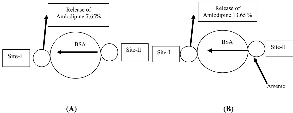
Fig 6. Proposed models of the Amlodipine-BSA- Arsenic interaction in absence of warfarin (site-I specific probe) (A) Normal condition of binding (B) Drug interaction in absence of probe
