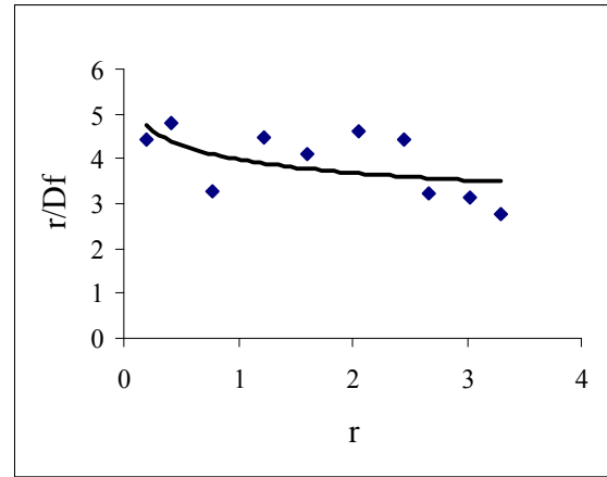
Fig 2. Scatchard plot for amlodipine bound to BSA at pH 6.4
